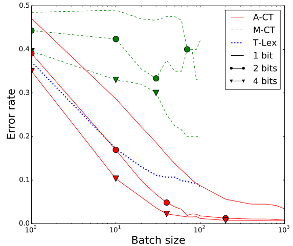
Figure 2: The effect of batch size on error rate. Batches of 100 are the maximum for M-CT and T-Lex, but we go up to 1000 with A-CT.
