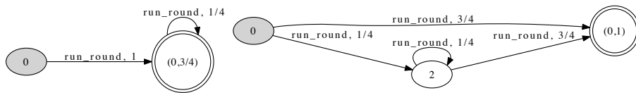
Fig. 4. Herman’s protocol: automata for early (left) and late (right) announcement.
