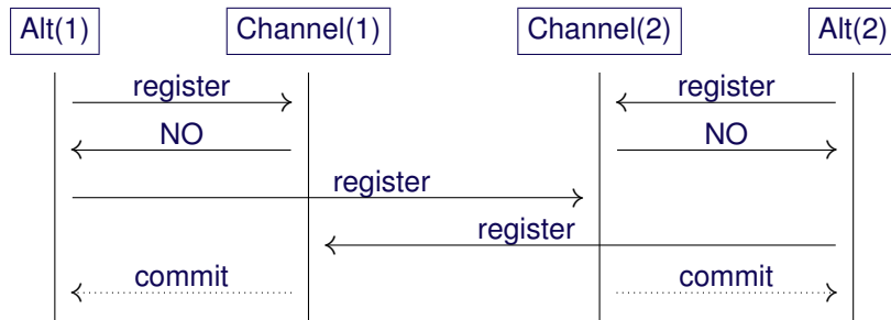
Figure 3. The behaviour leading to deadlock
