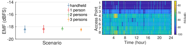
Figure 8: Nearby human body impact. Figure 9: Temporal variation of WiFi RSSI.
