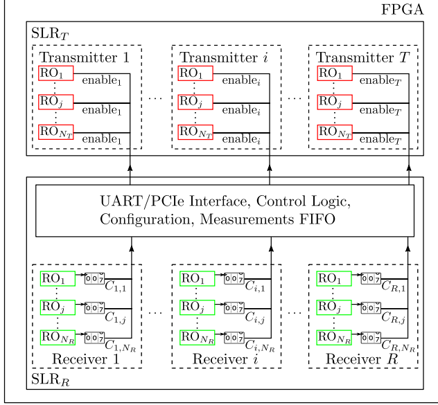
Fig. 3: Block diagram of the experimental setup, illustrating the logical and physical isolation of the R \cdot N_R RO receivers and the T \cdot N_T RO transmitters on separate SLRs.
