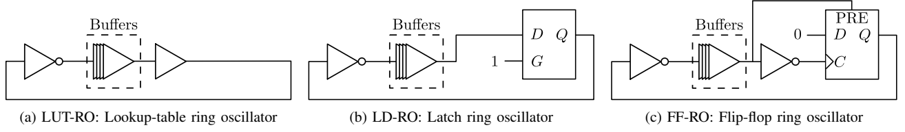
Fig. 4: Three ring oscillators designs with a variable number of intermediate buffer stages, used in local and cloud experiments. Although LUT-ROs (a) are prohibited on Amazon Web Services, LD-ROs (b) and FF-ROs (c) are not.
