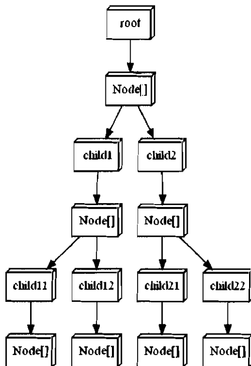
Figure 6.1: Initial, naive memory graph produced from the tree program.
