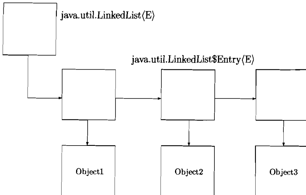
Figure 4.2: LinkedList before folding
