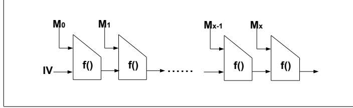
Figure 2.1: The Merkle-Damgård structure of conventional long-output cryptographic hash functions. Here f() is a one-way and collision-resistant compression function, IV is some public initial value, and the input message m is partitioned into multiple fixed-size blocks M_0, \dots, M_x , which are processed sequentially.
