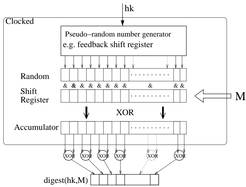
Figure 6.2: Hardware implementation of a digest function.
