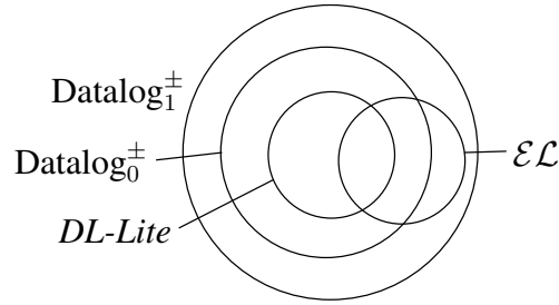
Figure 1: Relationships between \text{Datalog}_0^\pm , \text{Datalog}_1^\pm , DL\text{-Lite} , and \mathcal{EL} .
