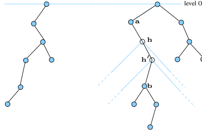
Figure 6: Construction in the proof of Lemma 4.
