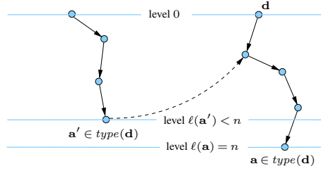
Figure 5: Construction in the proof of Lemma 3.
