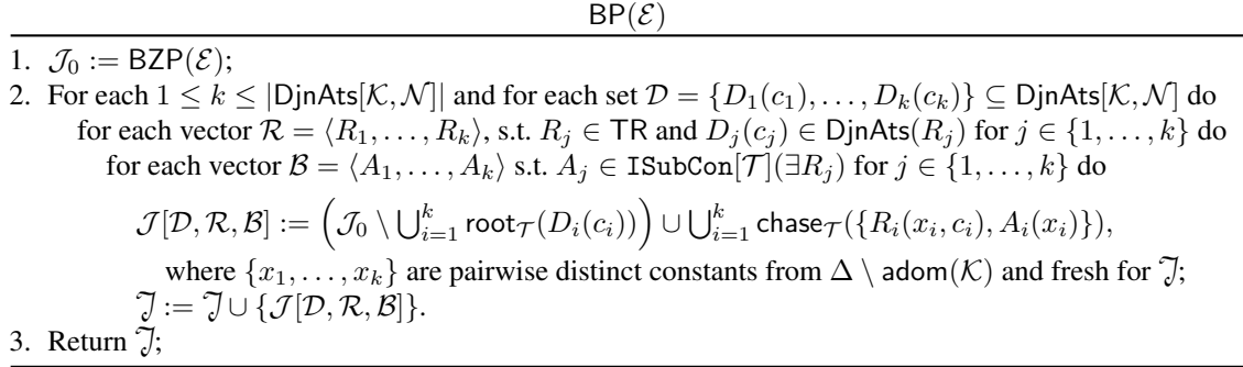
Figure 5.2. BP( \mathcal{E} ) procedure of building the prototypal set \mathcal{J} for a simple DL-Lite core -evolution setting \mathcal{E} = (\mathcal{K}, \mathcal{N}) with \mathcal{K} = \mathcal{T} \cup \mathcal{A}
