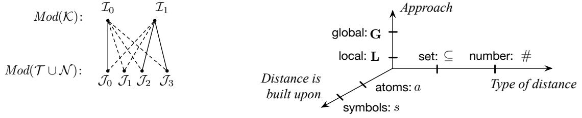
Figure 2.1. Left: measuring distances between models and finding local and global minima (Examples 2.7 and 2.9). Right: three-dimensional space of approaches to model-based evolution semantics.
