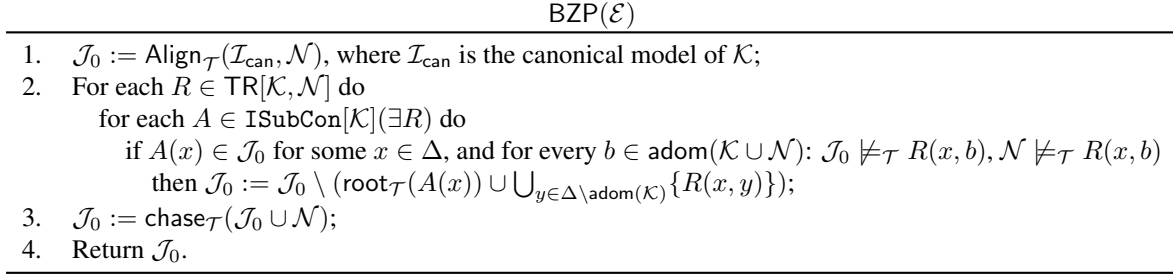
Figure 5.1. BZP( \mathcal{E} ) procedure for building the zero prototype \mathcal{J}_0 for a simple DL-Lite core -evolution setting \mathcal{E} = (\mathcal{K}, \mathcal{N}) where \mathcal{K} = \mathcal{T} \cup \mathcal{A}
