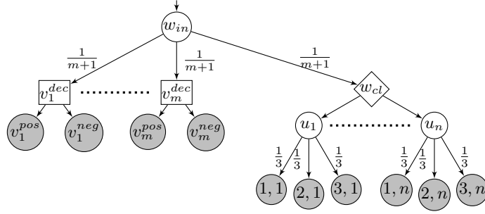
Fig. 6: Game illustrating NP-hardness. State label “ i, j ” corresponds to v_i^{pos} (resp. v_i^{neg} ) if the i th variable in clause c_j is positive (resp. negative).
