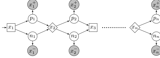
Fig. 5: Game illustrating PSPACE-hardness. Probabilities in stochastic states are uniform.
