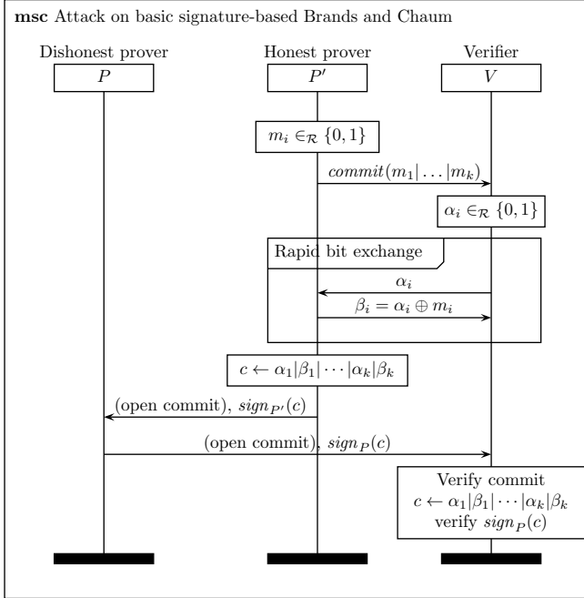
Figure 2. Distance Hijacking attack on basic signature-based Brands and Chaum. sign_P and sign_{P'} denote the signatures with the signature keys of P and P' , respectively.
