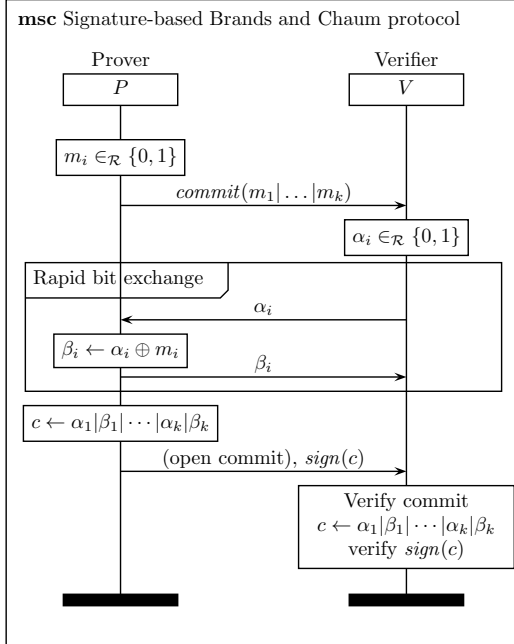
Figure 1. Signature-based Brands and Chaum protocol.
