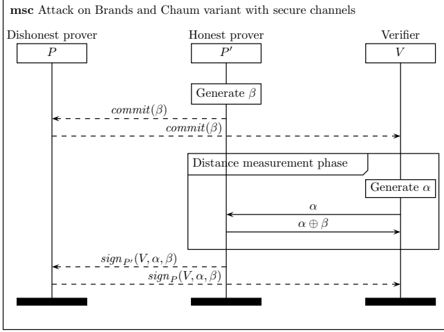
Figure 8. Attack on Brands and Chaum variant where setup and finalization use a secure channel. We use dashed arrows to denote transmission over a secure channel. P' assumes that P is a verifier.
