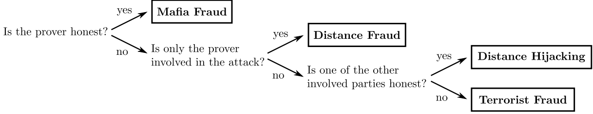
Figure 4. Classification of attacks on distance bounding protocols, in which a verifier computes an incorrect distance bound for a prover.
