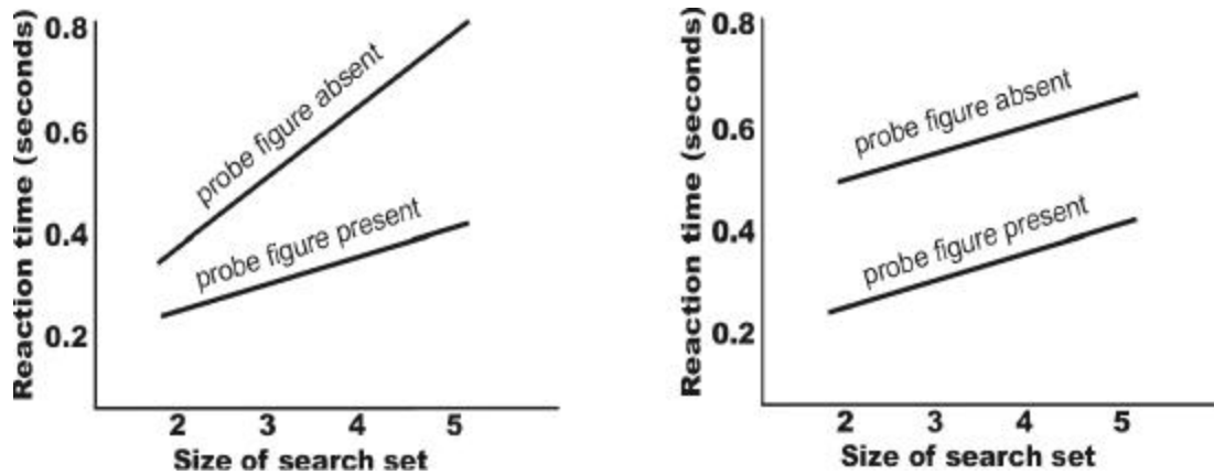
Figure 7: The graph on the left illustrates the results expected if search for the probe target was serial and self-terminating. The one on the right, which was the form actually found by Sternberg(1966), is what you would expect if the search was serial and exhaustive (i.e., continued even after the target was found).
