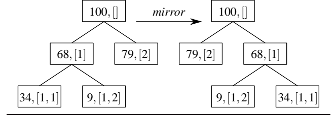
Figure 3. Using mirror as a ‘get’ function.
