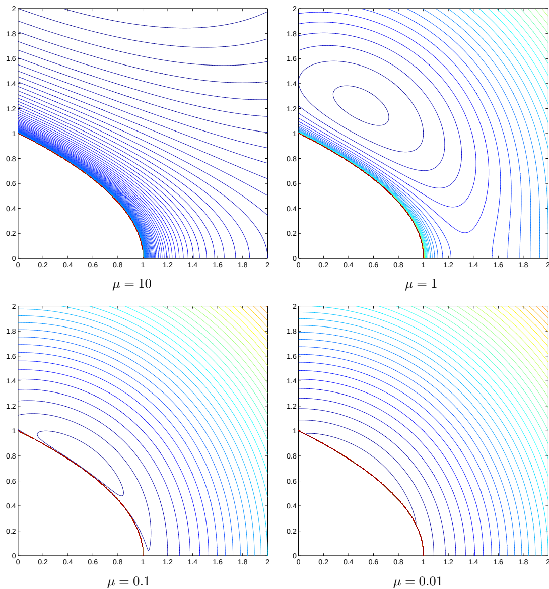
Figure 6.1: The logarithmic barrier function for \min x_1^2 + x_2^2 subject to x_1 + x_2^2 \geq 1 . The contours for \mu = 0.01 are visually indistinguishable from f(x) for feasible points.
