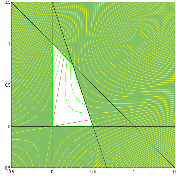
Figure 4.2: Another non-convex problem: contours of the objective function x_1^2 + x_2^2 - 6x_1x_2 and the feasible region for the constraints x_1 + x_2 \leq 1 , 3x_1 + x_2 \leq 1.5 and (x_1, x_2) \geq 0 . Note that escaping from the origin may be difficult!
