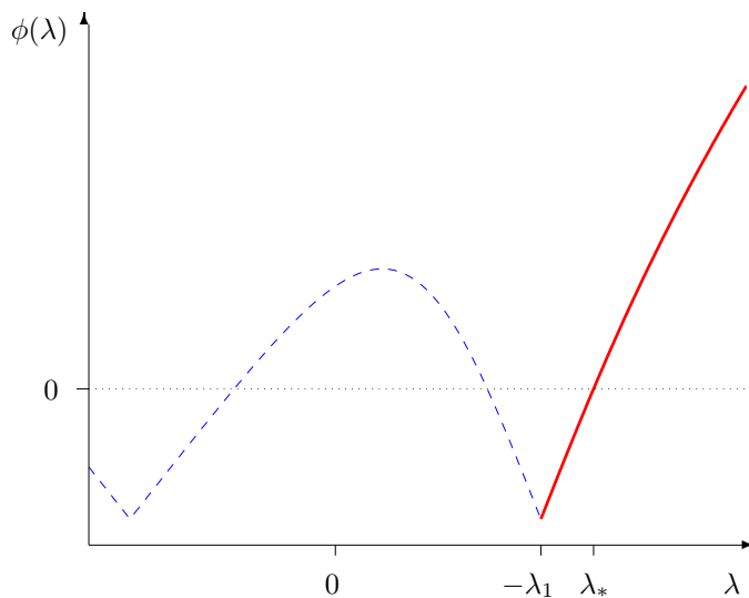
Figure 3.5: A plot of \phi(\lambda) against \lambda for the problem of minimizing -\frac{1}{4}s_1^2 + \frac{1}{4}s_2^2 + \frac{1}{2}s_1 + s_2 subject to \|s\|_2 \leq 4 .
