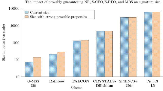
Figure 6: Provably achieving security properties beyond unforgeability for the NIST round 3 candidates: for candidates that do not provably offer these properties yet, our BUFF transformation slightly increases signature size. Since the additional size is constant (64 bytes), the largest relative increase occurs for the smallest signature size (e.g. GeMSS256 goes from 72 to 136 bytes); however, this not even impacts the relative ordering of candidates based on signature size. Since the BUFF transformation involves only a single hash, the additional computational cost is in all cases negligible compared to the signature generation and verification.
