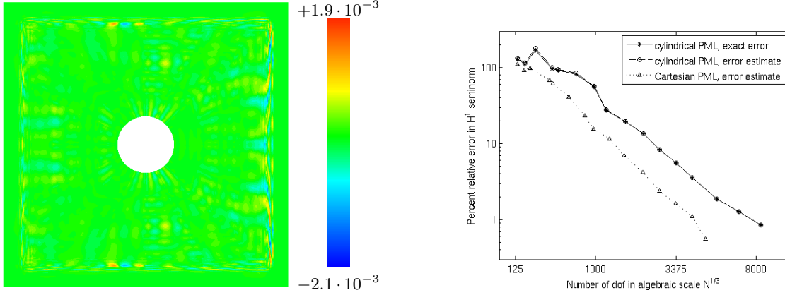
Figure 4: Acoustic scattering of a plane wave on a unit cylinder. Left : Real part of the error estimate for the case with Cartesian PML. Right : Percent relative error versus number of degrees-of-freedom for the cylindrical PML (exact error and error estimate) and for the Cartesian PML (error estimate).
