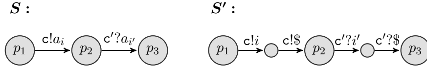
FIGURE 8. Simulating reliable channels (left) with “strict-superseding” or “overtaking” PCSs (right).
