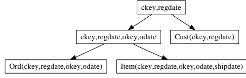
Figure 6: Tree representation of the FD-reduct of Example 3.18.
