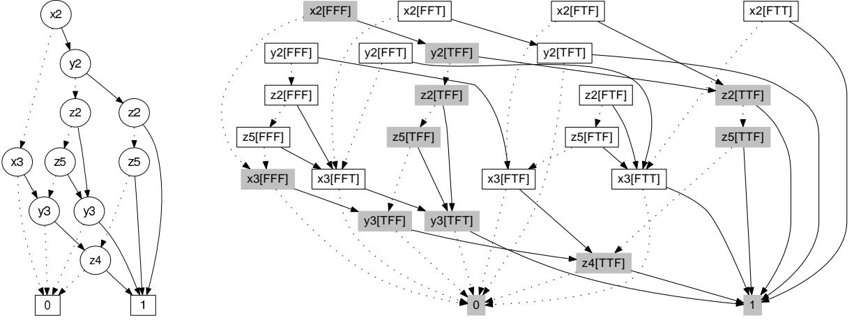
Left: Reduced OBDD used in Section 4. Right: Partially reduced OBDD as constructed by the algorithm of Section 5. Constant nodes are merged, and nodes z_4[FFF] , z_4[FTF] , z_4[TFF] , y_3[FFT] and y_3[FFF] are removed for compactness (although the algorithm constructs them). Grey nodes form the equivalent reduced OBDD on the left.
