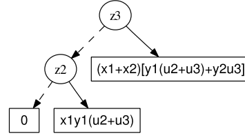
Figure 9: Partial OBDD used in Example 4.9.
