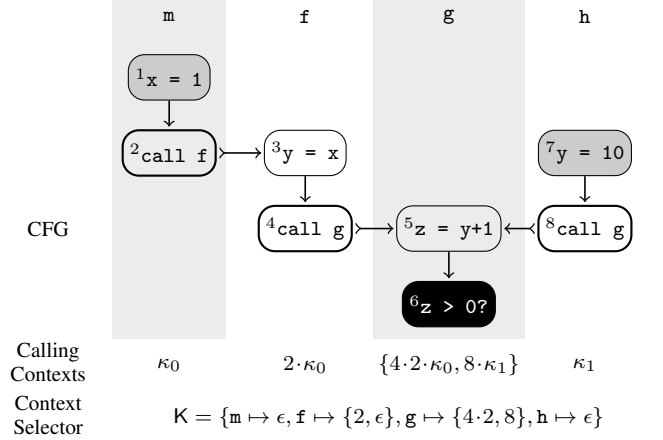
Figure 2. Example context selector. Gray and black nodes in CFG are source and query points, respectively.
