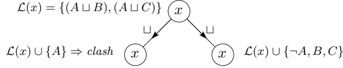
Fig. 9.7. Semantic branching search
