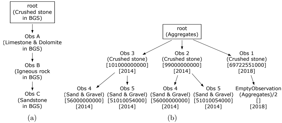
Figure 6: Examples of trees built by the PCSC “algorithm”. (a) and (b) show the trees corresponding to the examples in Figure 4c and Figure 5, respectively.
