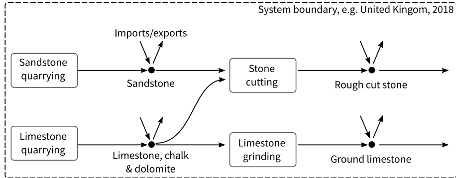
Figure 1: MEFA system showing rock processing stages in the UK. Processes are shown by boxes. The arrows represent flows. The types of materials are shown by dots, with the vertical flows representing trade flows across the system boundary.
