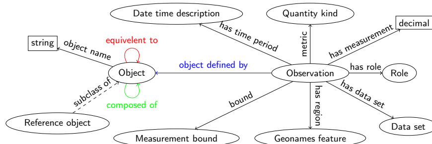
Figure 2: The core concepts and relations in the PRObs ontology.
