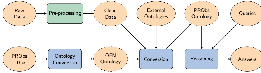
Figure 7: Back-end pipeline. The rectangles represent the steps of our pipeline (green for Python scripts and blue for RDFox scripts). The ellipses represent inputs and outputs (dashed for internal results).
