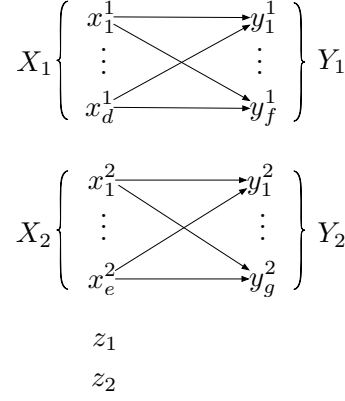
Fig. 4 Dependency graph for Proposition 2 ( X_1 = \{x_1^1, \dots, x_d^1\} , X_2 = \{x_1^2, \dots, x_e^2\} , Y_1 = \{y_1^1, \dots, y_f^1\} , and Y_2 = \{y_1^2, \dots, y_g^2\} ).
