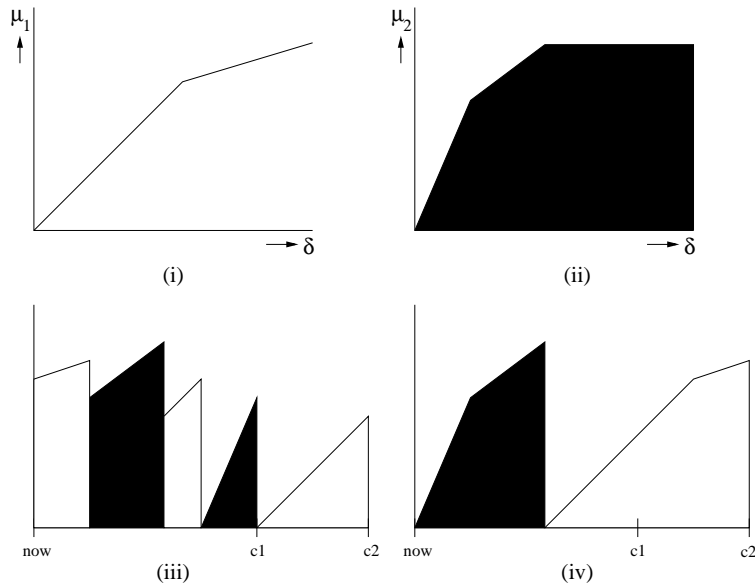
Figure 1: A simple example of continuous deliberation scheduling (from [BD94]). Assume that an agent has two future events, c_1 and c_2 , to respond to, and aims to maximise the value of both responses. The agent has at its disposal decision procedures for responding to events c_1 and c_2 . In (i) and (ii) the respective performance profiles of these decision procedures are shown. Such a performance profile defines the expected response value ( \mu_c ) as a function of the allocated time ( \delta ) for that decision procedure. Panel (iii) shows the allocation of time for the respective decision procedures, resulting from the continuous deliberation scheduling algorithm. Panel (iv) shows the final deliberation schedule, after collecting and sorting the timeslices.
