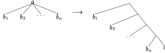
Fig. 7. Isomorphism between rose trees and leaf-labelled binary trees
