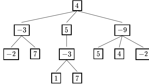
Fig. 2. A rose tree
