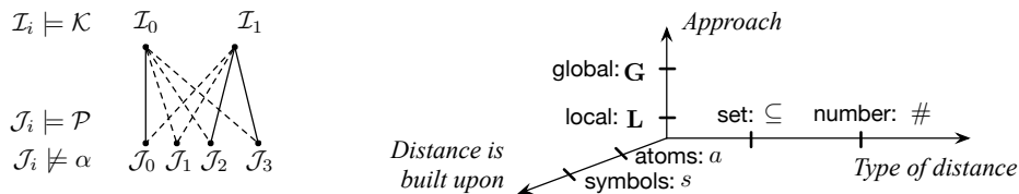
Fig. 2. Model-based contraction semantics: example and notation.
