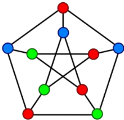
Colouring of the Peterson graph (source: Wikipedia).
