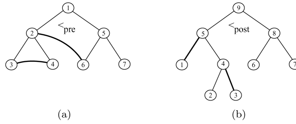
FIG. 3. (a) Following does not have the \underline{X} -property with respect to <_{pre} ; (b) Descendant^{-1} and Descendant-or-self^{-1} do not have the \underline{X} -property with respect to <_{post} .
