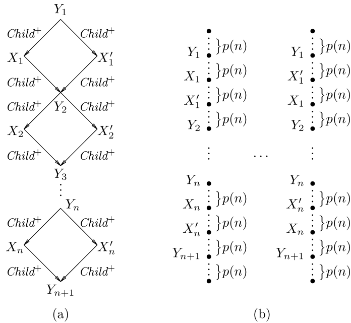
FIG. 9. (a) Query D_n (b) and path structures PS(n, p(n)) .
