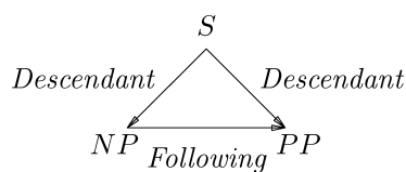
FIG. 1. A query graph.
