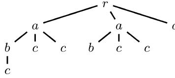
FIG. 2. A labeled tree.
