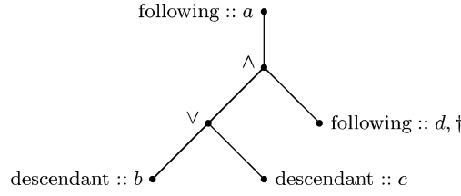
FIG. 7. Query-tree for expression following :: a[descendant :: b or descendant :: c]/following :: d.
