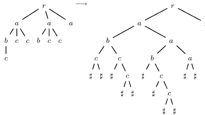
FIG. 10. From unranked to ranked trees.
