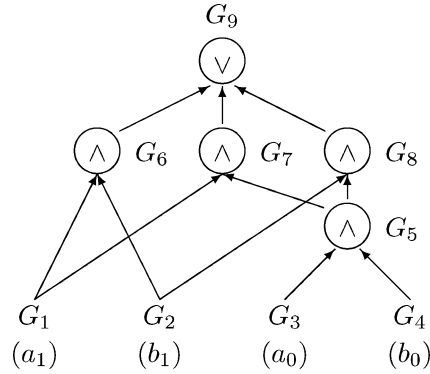
FIG. 3. A 2-bit full adder carry-bit circuit.
