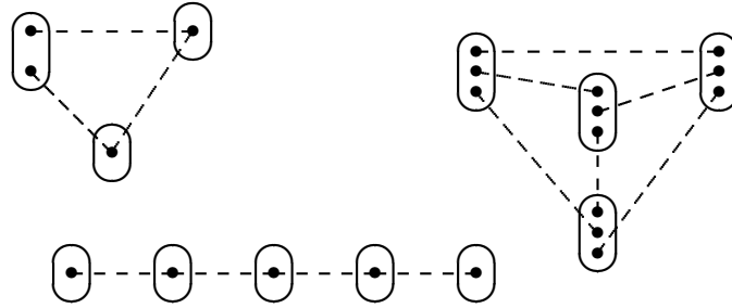
Figure 16: Three patterns whose topological-minor tractability is open.
