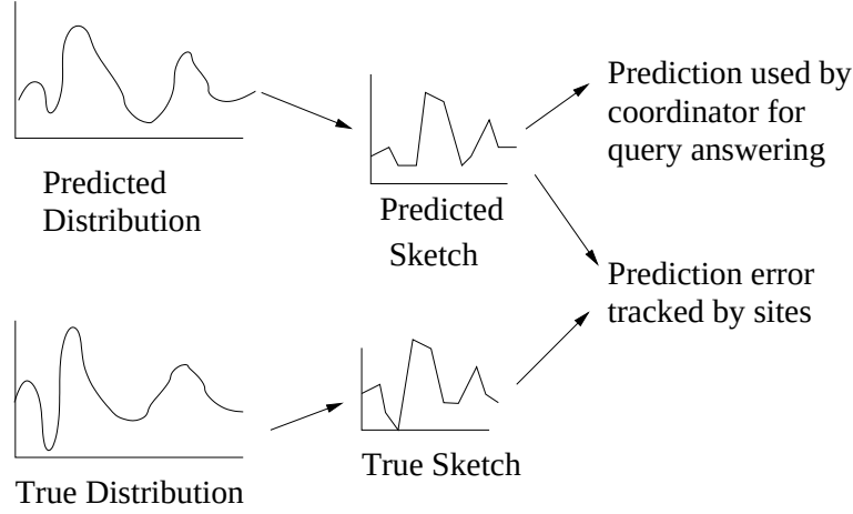
Fig. 2. Schematic of Sketch-Prediction-Based Tracking.
