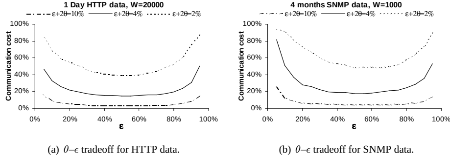
Fig. 6. Tradeoff between the parameters \epsilon and \theta .
