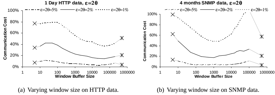
Fig. 7. Effect of varying the window size used to estimate the “velocity” sketch.
