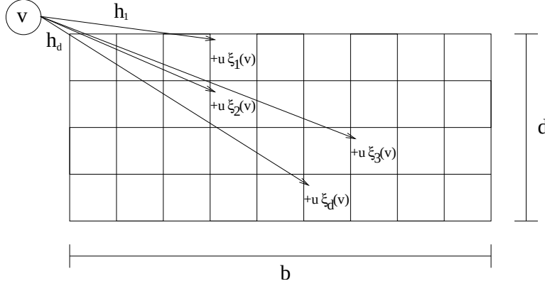
Fig. 4. Structure of the Fast-AGMS Sketch Summary.
