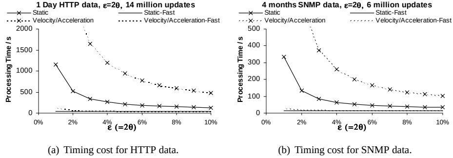
Fig. 10. Timing cost, comparing fast tracking methods to performing sketch estimation every step, for static and acceleration models.
