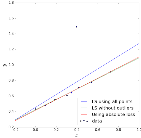
Figure 3: Least Squares Estimate is not robust to outliers.
