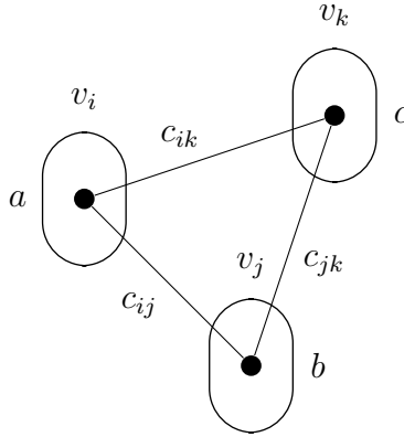
Figure 3: The joint-winner property: c_{ij}(a, b) \geq \min(c_{ik}(a, c), c_{jk}(b, c)) .
